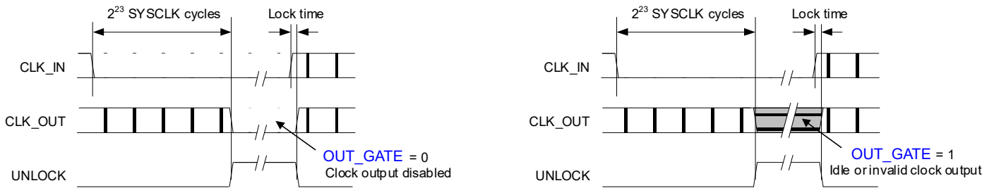
Figure 4-5. CLK_IN Interruption > 2^{23} SYSCLK Cycles
